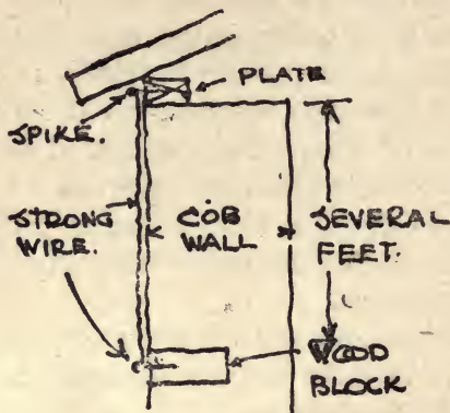
WALL COPINGS.
